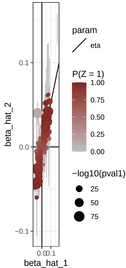
Sharing Model
