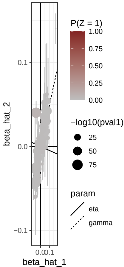
Causal Model
